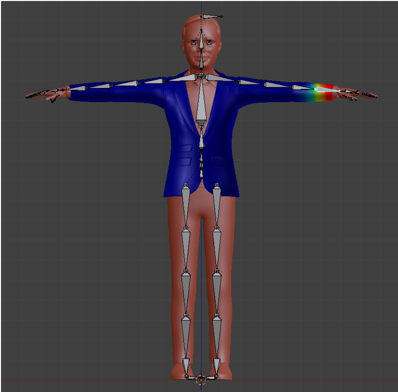
Illustration 1: Weight Painting
